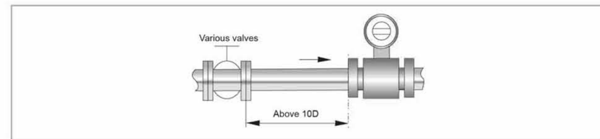
Minimum Length of Required Straight Pipe Segment
